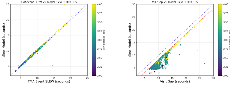
Figure 4. The slew model could accurately predict the time required to move the Simonyi Telescope Mount Assembly in altitude and azimuth, as shown by this comparison from a period during the SV survey, 2025-07-01 to 2025-07-10. However, the slew model was still somewhat inaccurate in predicting the entire visit gap. The offset of 1.6 seconds shown by the dotted red line can be explained by time required to configure and run scripts to execute the next step in the slew, but the scatter from that offset out to about 13.5 seconds is less clear. Similar tests run during the preLSST early operations phase show similar behavior.
