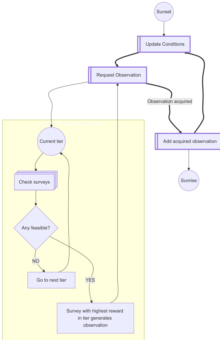
Figure 3. When the FBS is active, it continually cycles through the process of ingesting telemetry about the observatory conditions, returning requests for observations, and then ingesting information about acquired observations. When choosing observations in response to a request, the CoreScheduler iterates through the configured surveys. These surveys are arranged into tiers; surveys only compete within their own tier. If any survey within a given tier finds feasible observations, those observations will be chosen over any surveys in lower-ranking tiers. Within a given tier, the survey with the highest reward will request observations.
