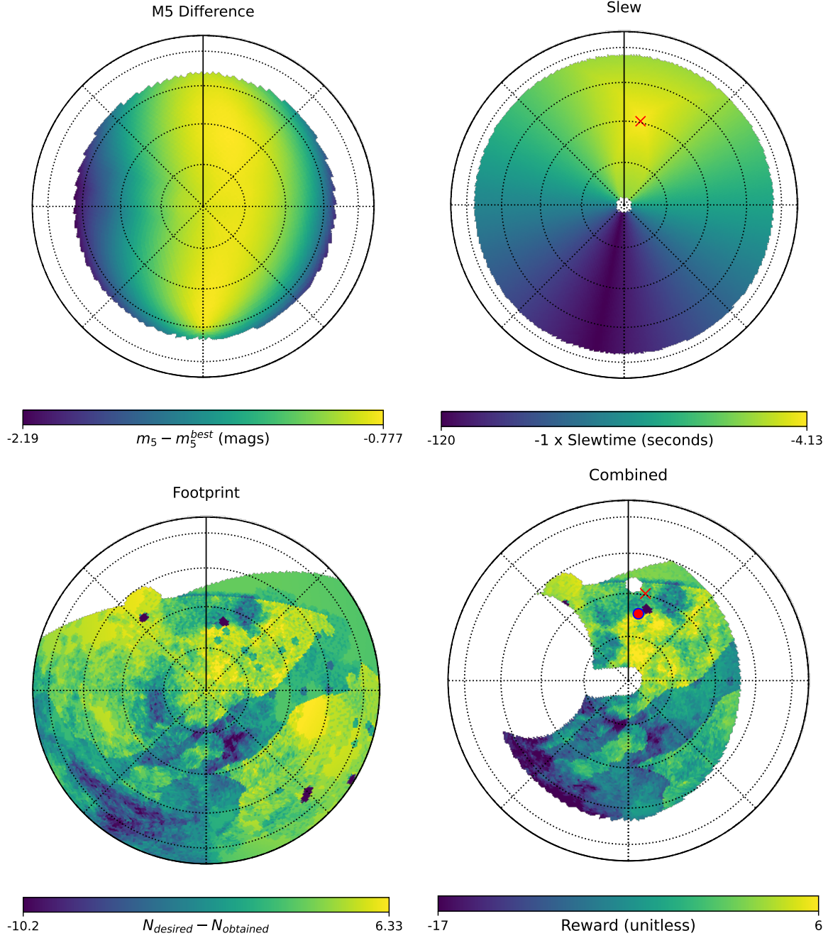
Figure 1. The primary basis functions to balance 5\sigma point source limiting magnitude( m_5 depth), uniform coverage, and on-sky efficiency are the M5DiffBasisFuntion, the SlewBasisFunction, and the FootprintBasisFunction, shown in the first three panels respectively. The stripe across the FootprintBasisFunction corresponds with the Galactic Plane, where the number of desired observations in this bandpass is lower than in the adjacent areas. These are alt-az plots, with zenith at the center. In the SlewBasisFunction, the red X marks the current pointing of the telescope. These, combined with additional basis functions to fine tune survey visit choices and including the standard masks from Figure 2, are shown in the final, “Combined” panel. The final panel also shows the next pointing that would be chosen by this survey, as a red circle.
